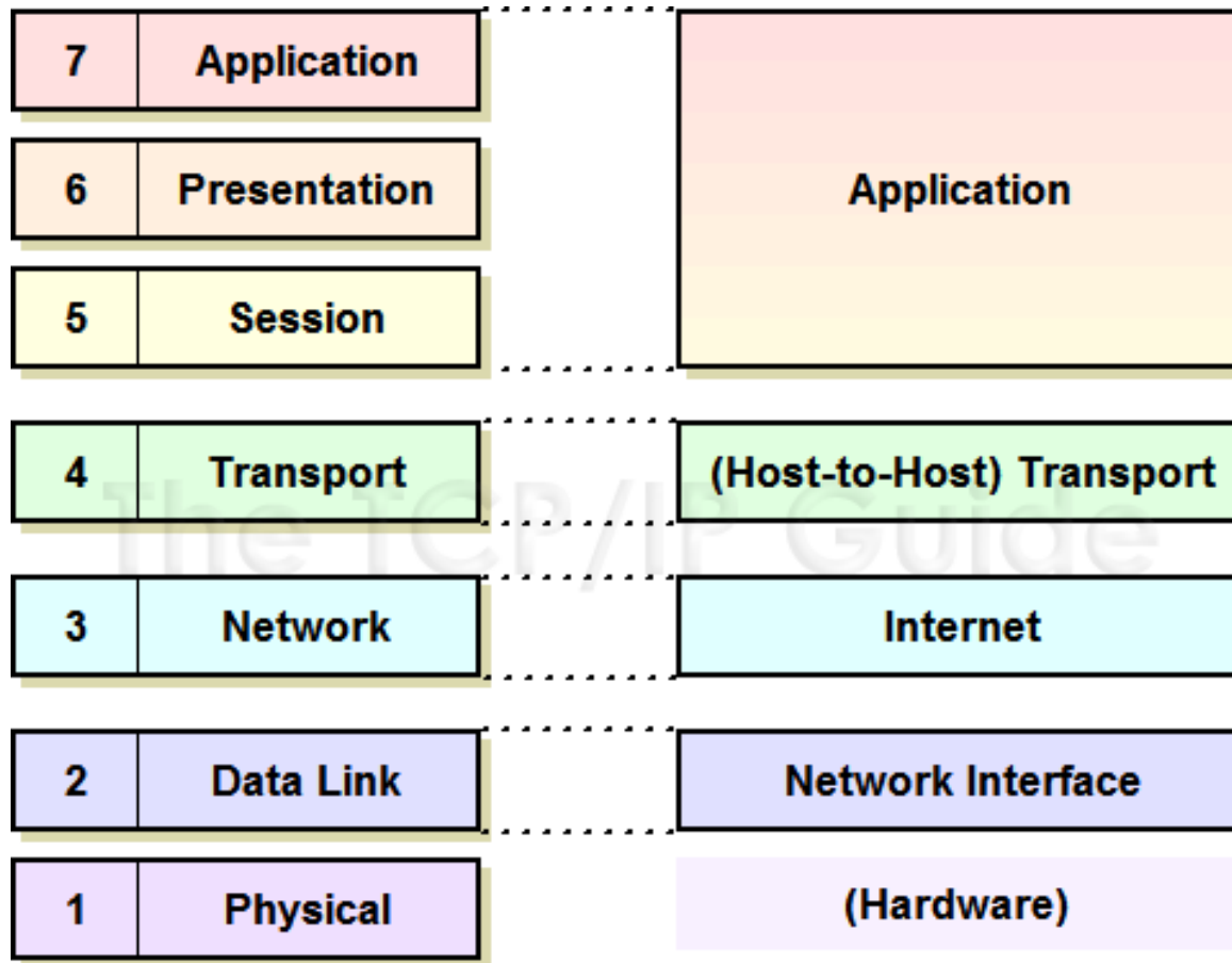
OSI Model
